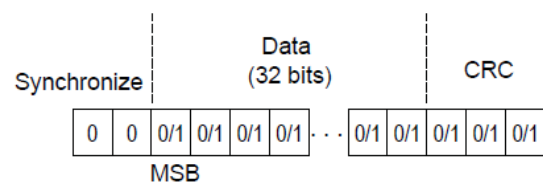
Figure 30: Read Acknowledge Sequence
