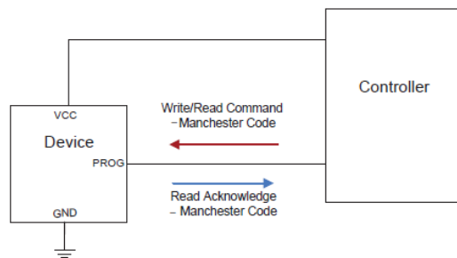
Figure 27: Programming Connections
