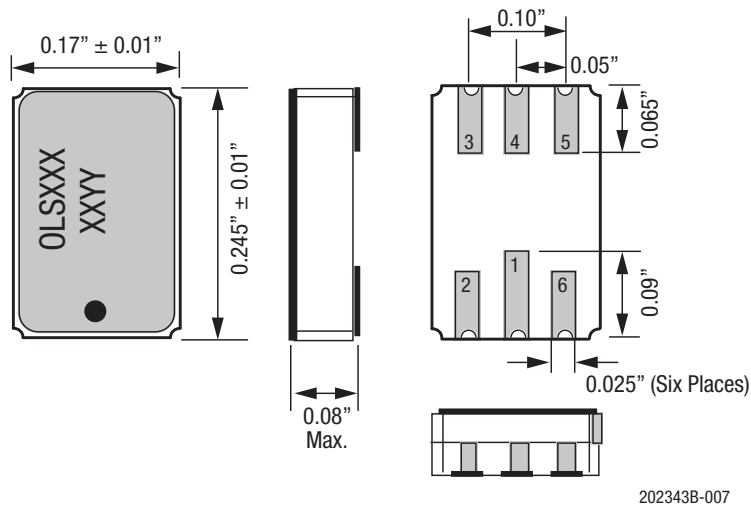
Figure 7. OLS400 Package Dimensions
