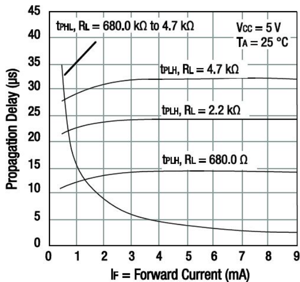
Figure 4. Propagation Delay vs Input Diode Forward Current
