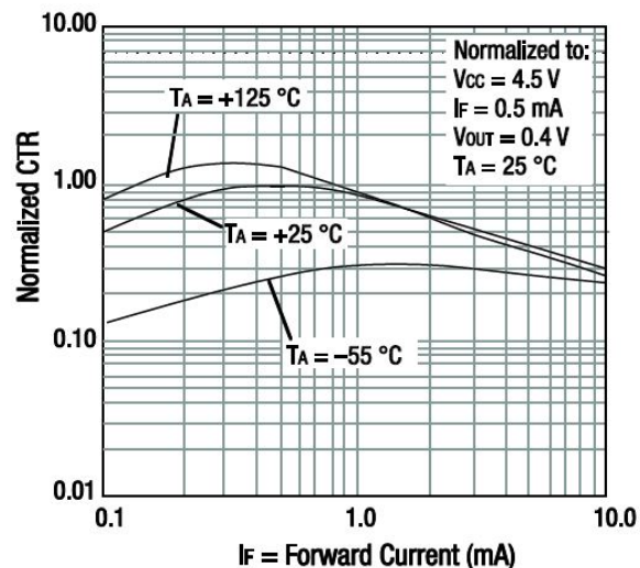
Figure 3. Normalized CTR vs Input Diode Forward Current
