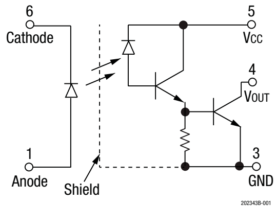
Figure 1. OLS400 Block Diagram
