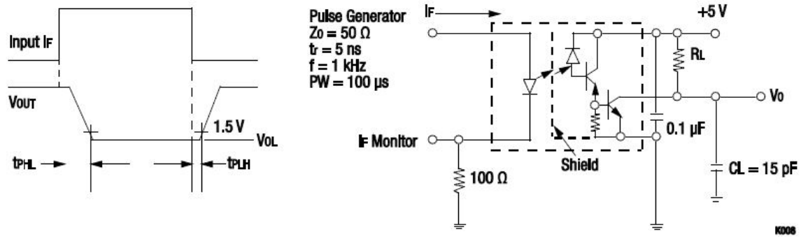
Figure 6. OLS400 Switching Test Circuit
