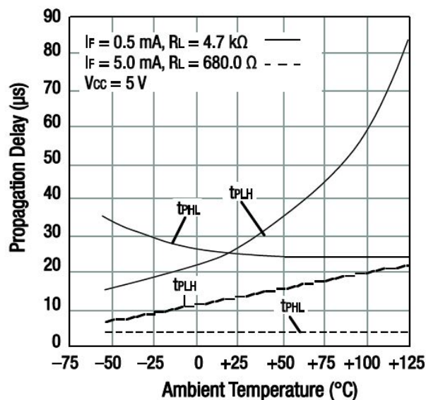
Figure 5. Propagation Delay vs Temperature
