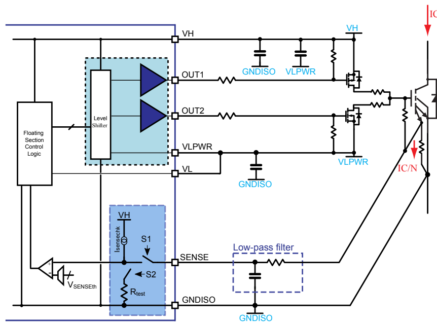
Figure 41. SENSE comparator check
