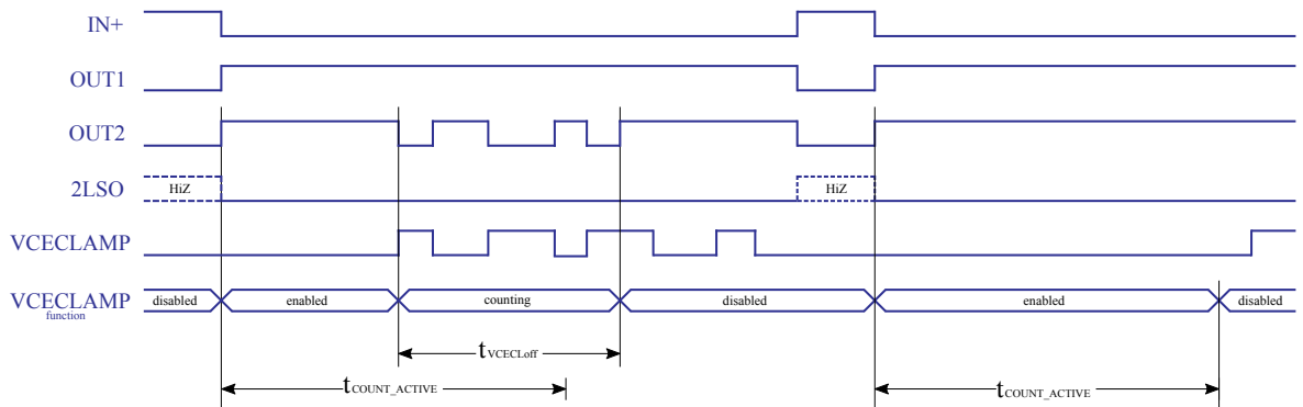
Figure 32. VCECLAMP activation (OFFMODE = '0')
