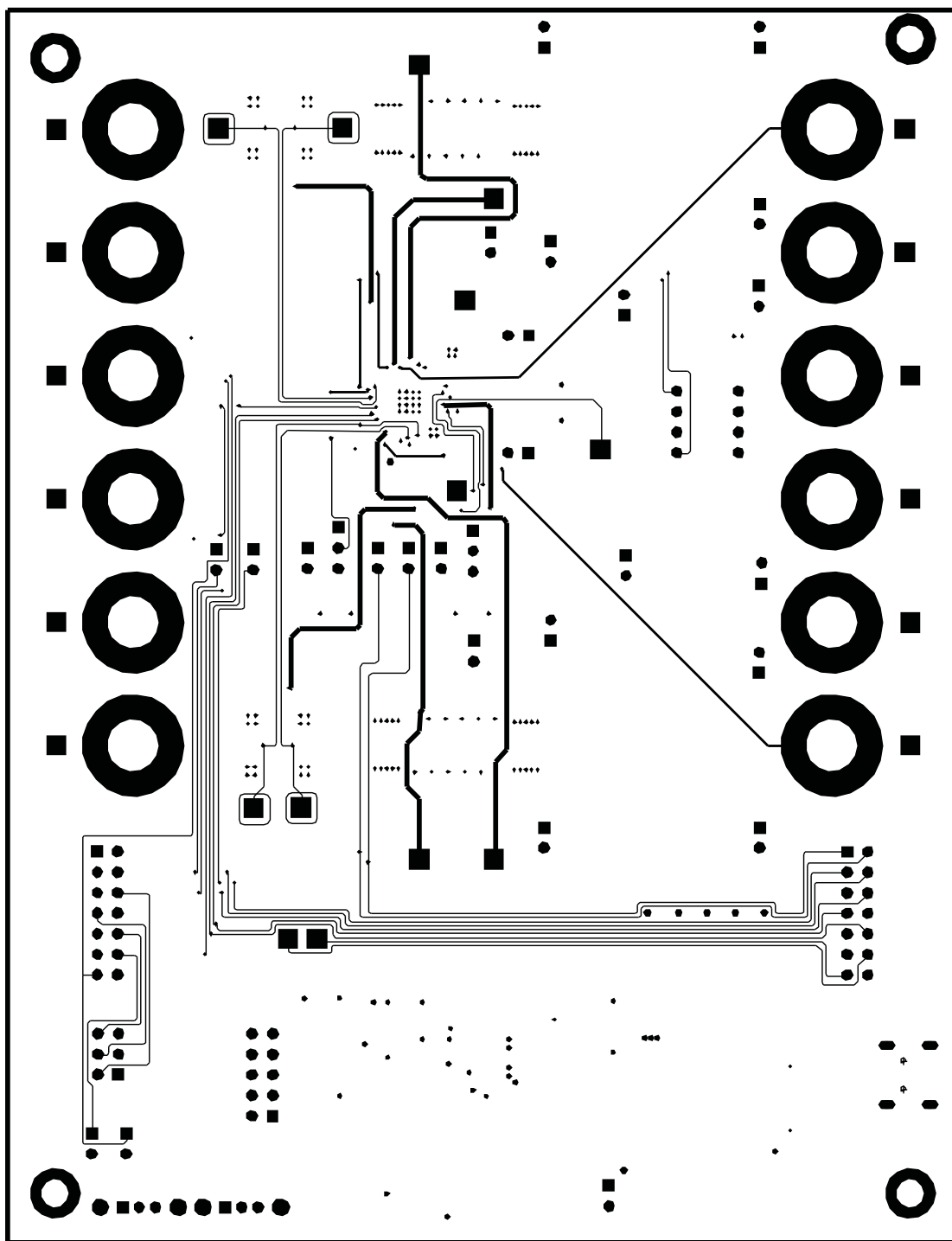
Figure 14. PCB Layer 3
