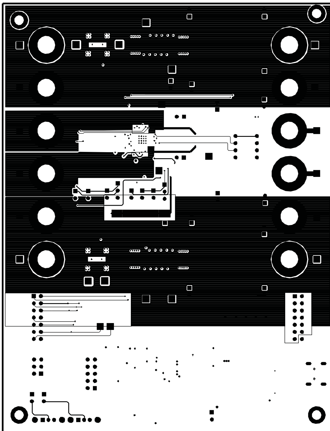
Figure 13. PCB Layer 2
