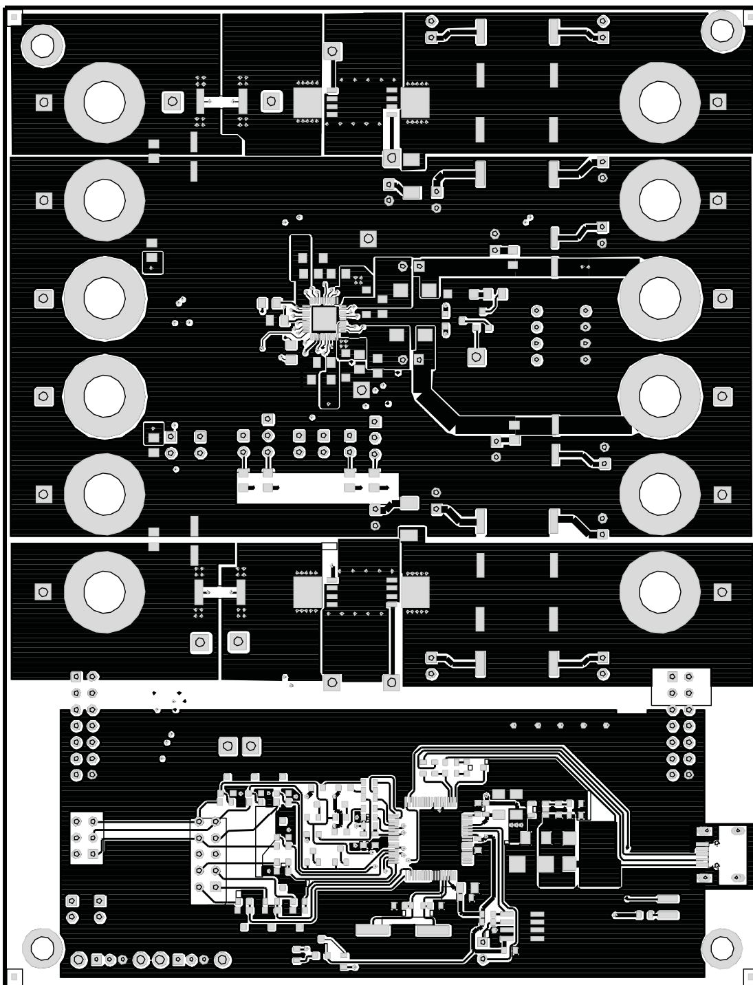
Figure 12. PCB Top Layer
