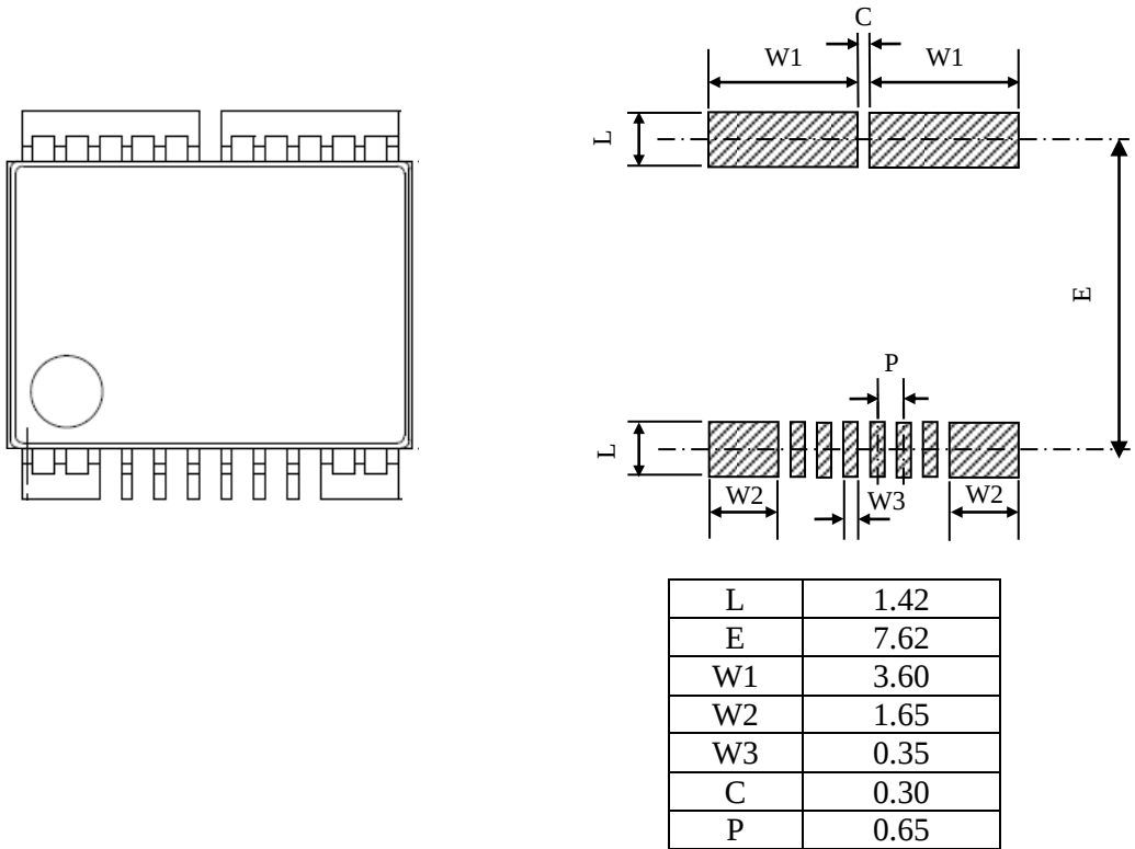
Figure 10. Pad dimensions of CQ-320A.
