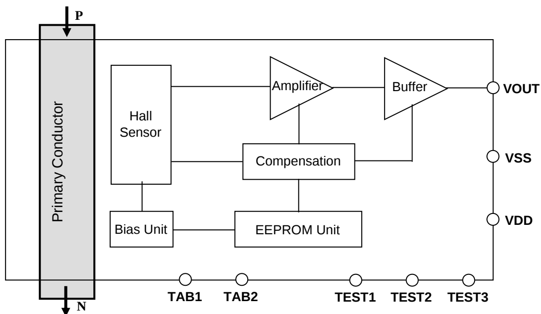
Figure 1. Functional block diagram of CQ-320A.
