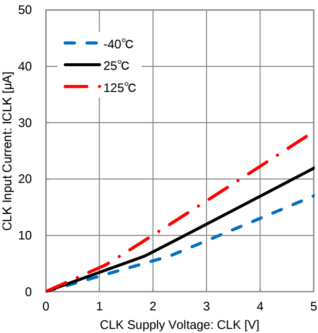
Figure 33. CLK Input Current vs CLK Supply Voltage (CLK Inflow Current)
