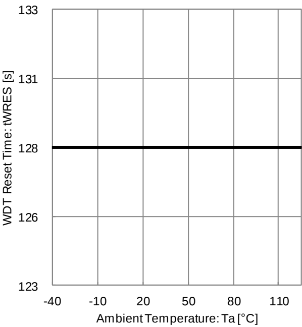
Figure 31. WDT Reset Time vs Ambient Temperature (WDT Reset Time)
