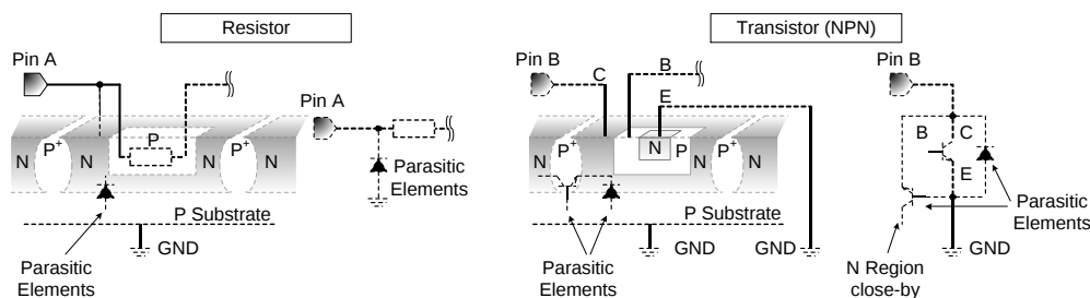
Example of monolithic IC structure
