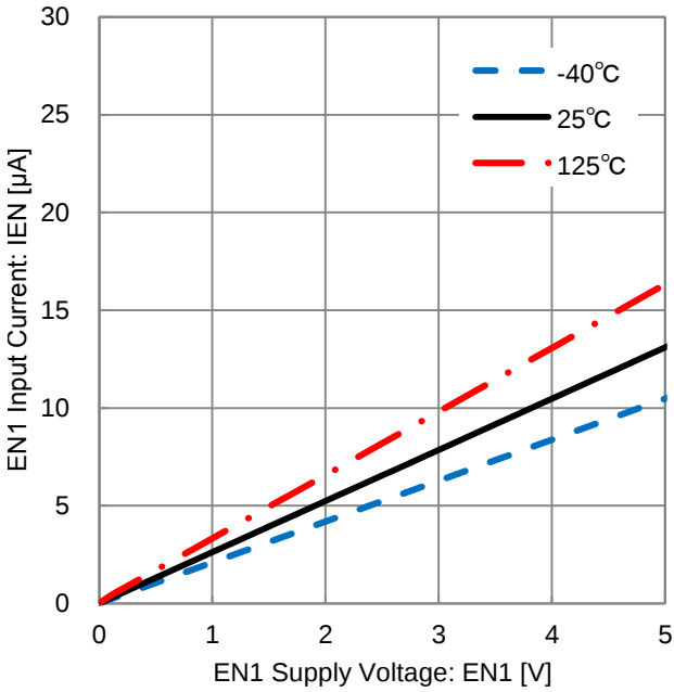
Figure 9. EN1 Input Current vs EN1 Supply Voltage (EN Inflow Current)
