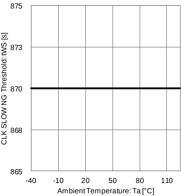
Figure 30. CLK SLOW NG Threshold vs Ambient Temperature (CLK SLOW NG Threshold)
