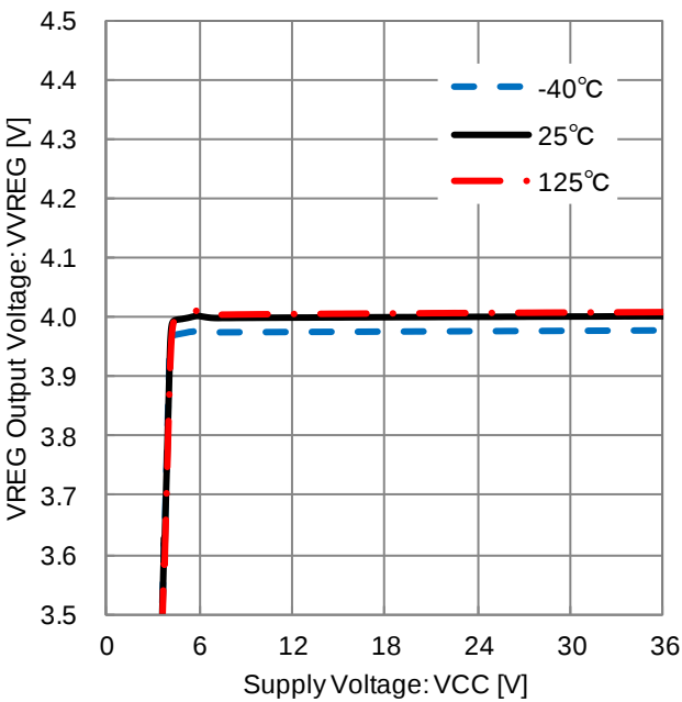
Figure 7. VREG Output Voltage vs Supply Voltage (VREG Output Voltage)
