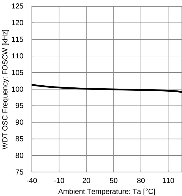
Figure 28. WDT OSC Frequency vs Ambient Temperature (WDT Oscillation Frequency)
