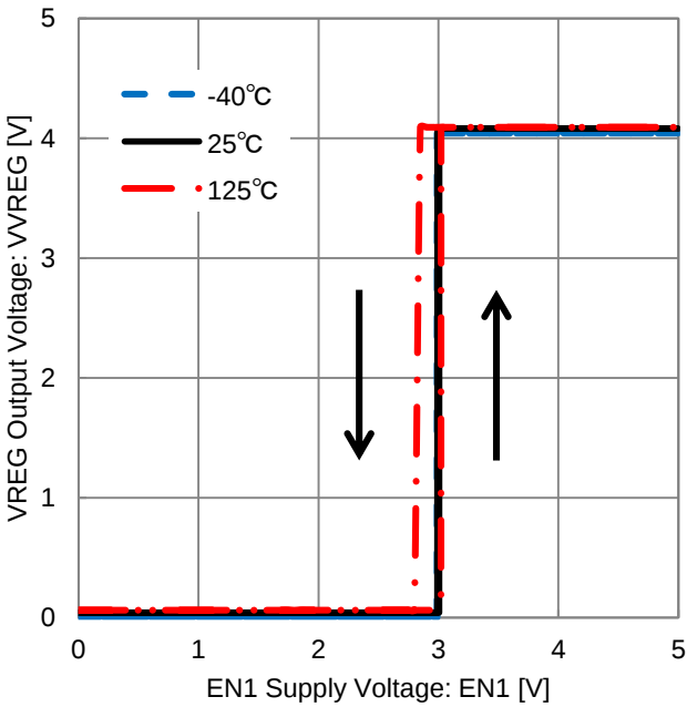
Figure 8. VREG Output Voltage vs EN1 Supply Voltage (EN Threshold Voltage)
