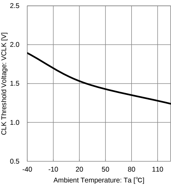
Figure 32. CLK Threshold Voltage vs Ambient Temperature (CLK Threshold Voltage)
