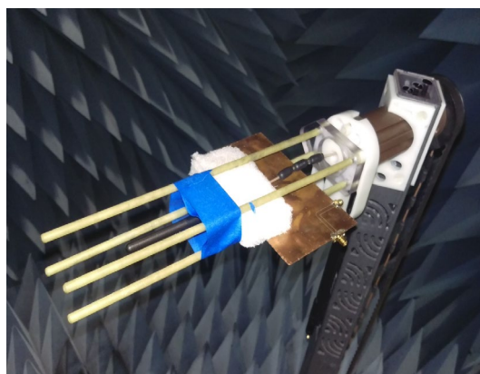
15cm x 9cm Ground Plane Edge
