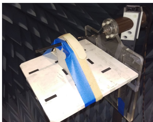
30mm x 30mm Ground Plane Center
