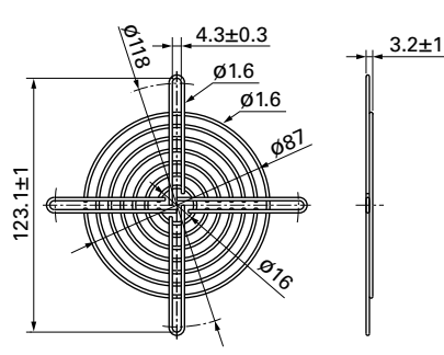
Inlet side
