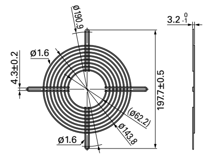
Outlet side
