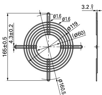
Outlet side
