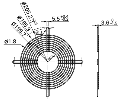
Outlet side
