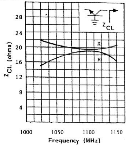
TYPICAL COLLECTOR LOAD IMPEDANCE vs. FREQUENCY
