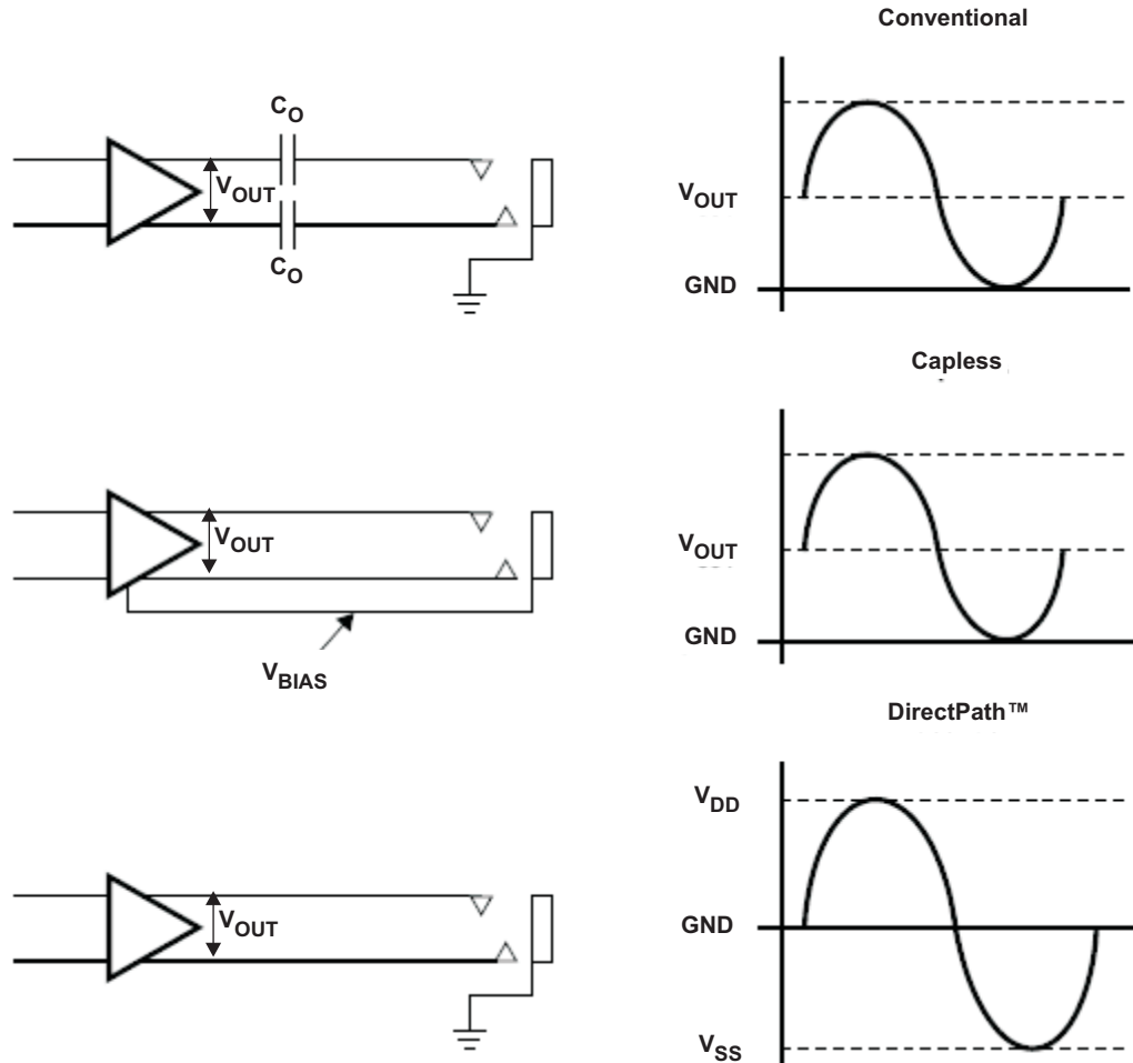
Figure 31. Amplifier Applications
