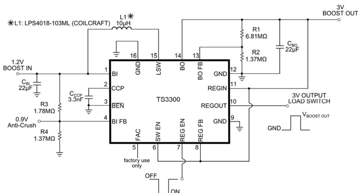
Figure 1. Boost + Output Load Switch Circuit Configuration
