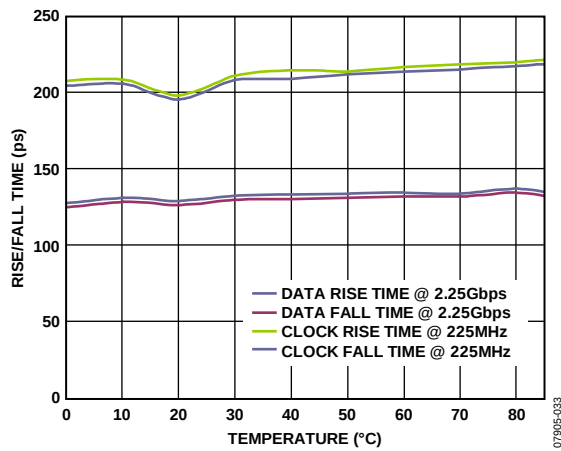
Figure 19. Rise/Fall Time vs. Temperature
