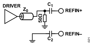
Figure 21. Reference Input Single-Ended Diagram
