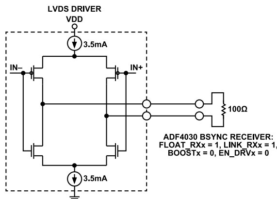
Figure 39. LVDS Driver to ADF4030 BSYNC Receiver Connection
