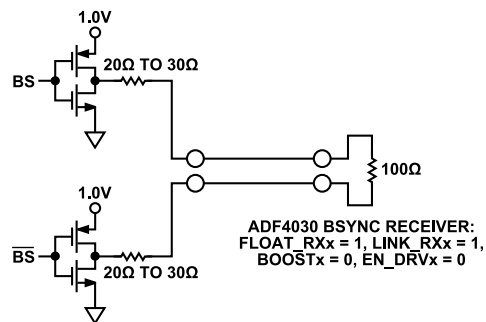
Figure 37. AD9084/AD9088 SYSREF to ADF4030 BSYNC Connection
