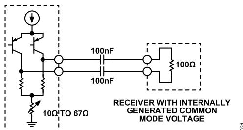
Figure 31. Differential Voltage Driver, AC-Coupled, 100\ \Omega Termination at Receiver
