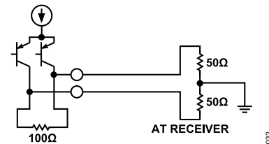
Figure 32. Differential Current Driver, Terminated, DC-Coupled 50\ \Omega to Ground Terminations at Receiver
