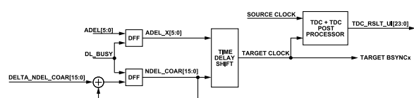
Figure 52. Open-Loop Delay Adjustment Process
