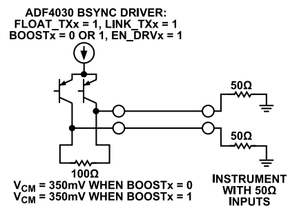
Figure 40. ADF4030 BSYNC Driver to 50 \Omega Instrument Connection
