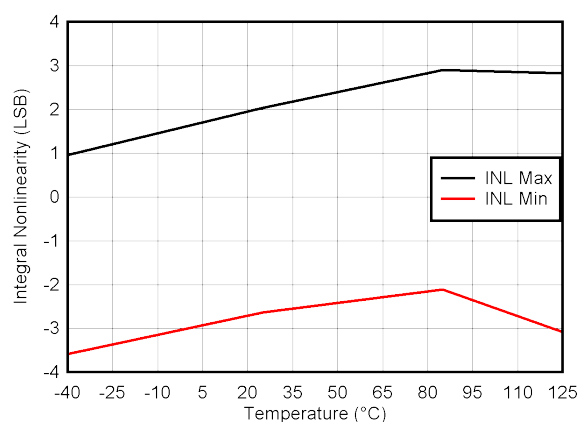
Figure 6-31. ADC INL Range vs Temperature
