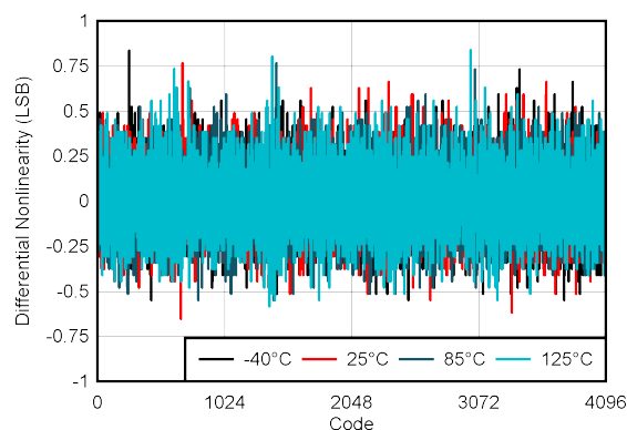
Figure 6-28. ADC DNL vs Digital Input Code
