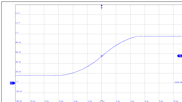
Figure 7-5. Sinusoidal Slew Rate: Rising
