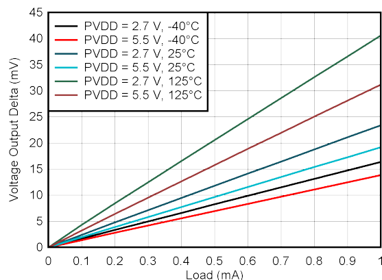
Figure 6-9. Zero-code Impedance
