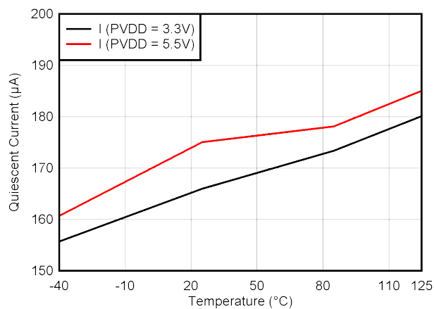
Figure 6-44. PVDD Supply Current vs Temperature
