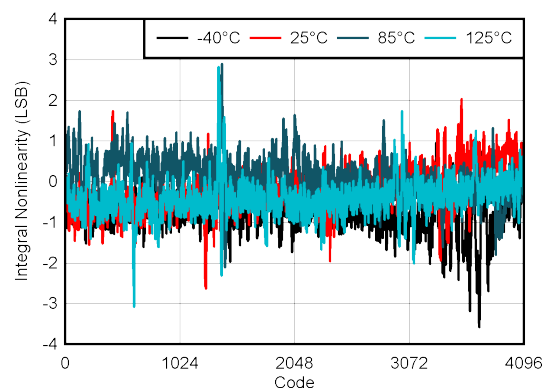
Figure 6-29. ADC INL vs Digital Input Code
