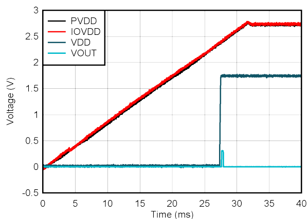
Figure 6-26. DAC Supply Power On, PVDD = 2.7\text{ V}
