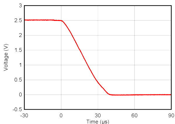
Figure 6-22. DAC Falling Settling Time
