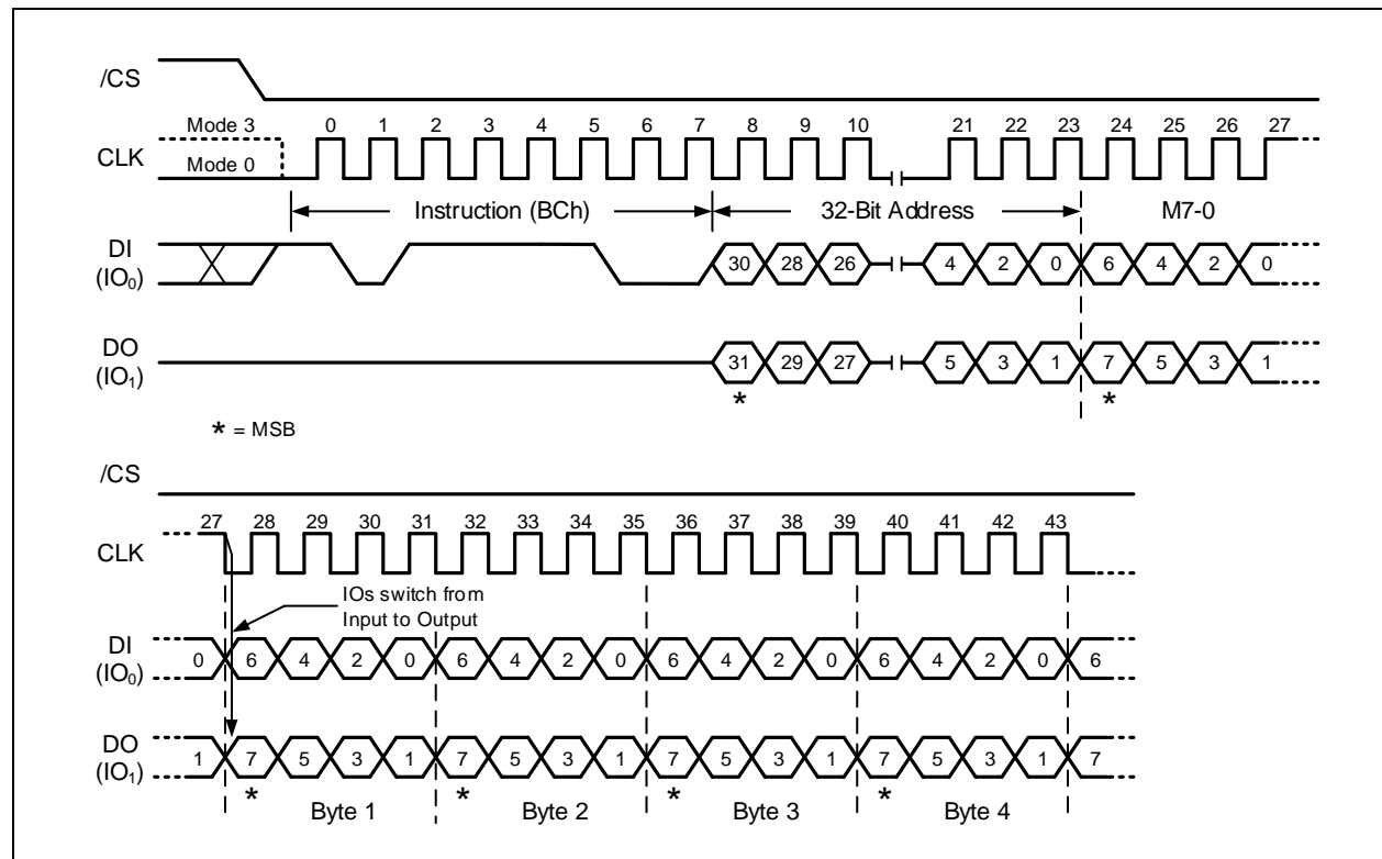
Figure 25a. Fast Read Dual I/O w/ 4-Byte Addr. (M7-M0 should set to Fxh, SPI Mode only)
