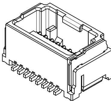
16-24極 16-24 CIRCUIT
