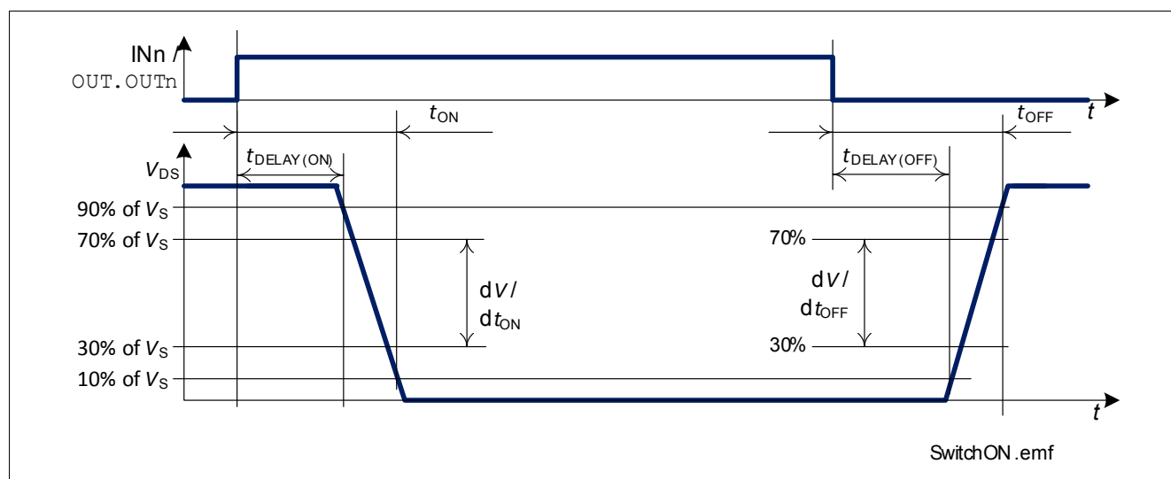
Figure 15 Switching a Resistive Load
