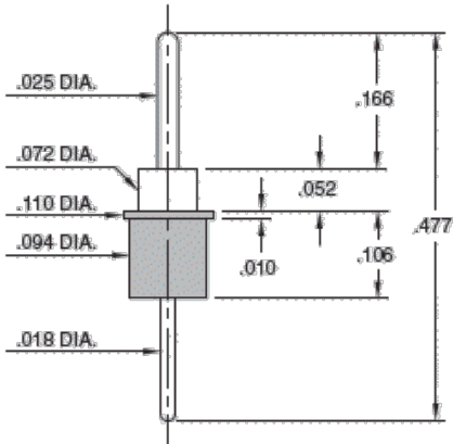
302-10-001-00-900800 Through-hole mount pin with insulated sleeve
