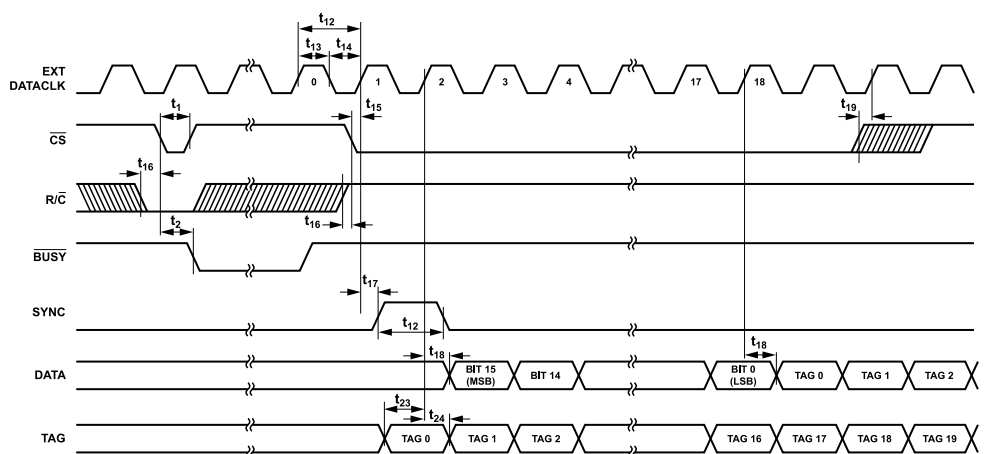
Figure 11. Conversion and Read Timing Using an External Continuous Data Clock ( \overline{EXT}/\overline{INT} Set to Logic High)
