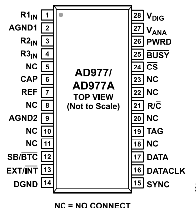
Figure 4. SSOP
