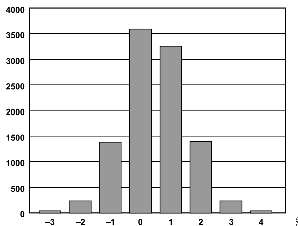
Figure 30. Histogram of 10,000 Conversions of a DC Input
