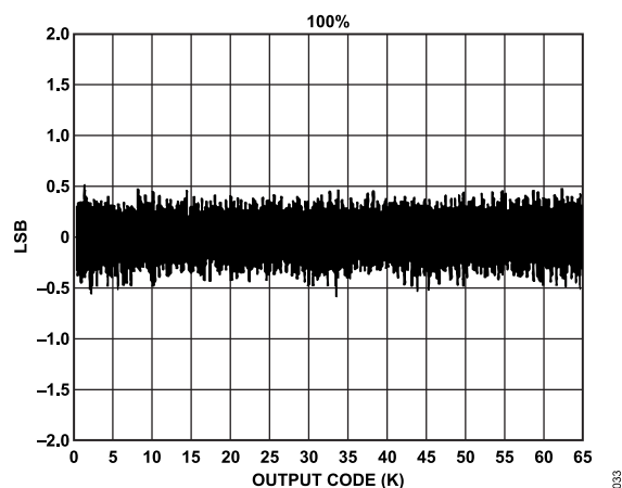
Figure 23. DNL Plot
