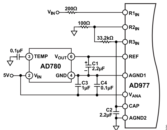
Figure 19. AD780 External Reference to AD977 Configured for \pm 10\text{ V} Input Range
