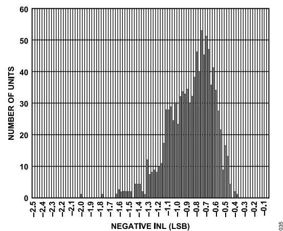
Figure 25. Typical Negative INL Distribution (999 Units)
