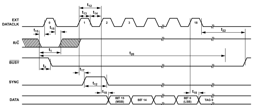
Figure 10. Conversion and Read Timing for Reading Previous Conversion Results During a Conversion Using External Discontinuous Data Clock (EXT/INT Set to Logic High, CS Set to Logic Low)
