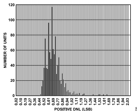
Figure 26. Typical Positive DNL Distribution (999 Units)
