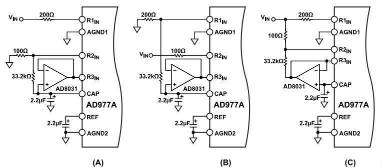
Figure 14. AD977A Bipolar Input Configuration Using the Internal Reference; (a) V_{IN} = \pm 10 V, (b) V_{IN} = \pm 5 V, (c) V_{IN} = \pm 3.33 V
