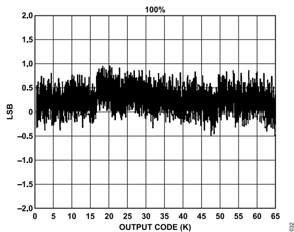
Figure 22. INL Plot
