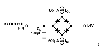
Figure 2. Load Circuit for Digital Interface Timing
