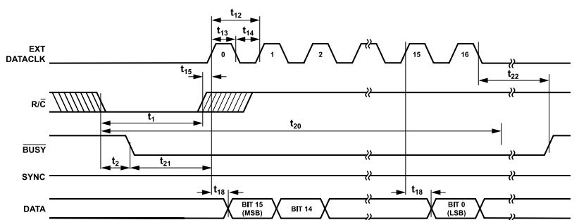
Figure 8. Conversion and Read Timing for Reading Previous Conversion Results During A Conversion Using External Discontinuous Data Clock ( \text{EXT}/\overline{\text{INT}} Set to Logic High, \overline{\text{CS}} Set to Logic Low)
