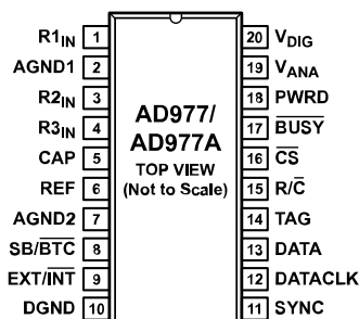
Figure 3. SOIC
