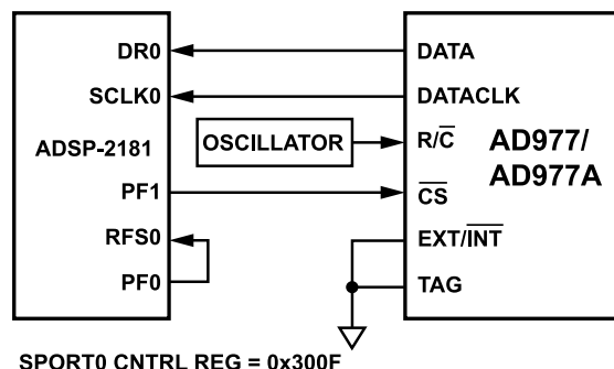
Figure 34. AD977/AD977A to ADSP-2181 Interface
