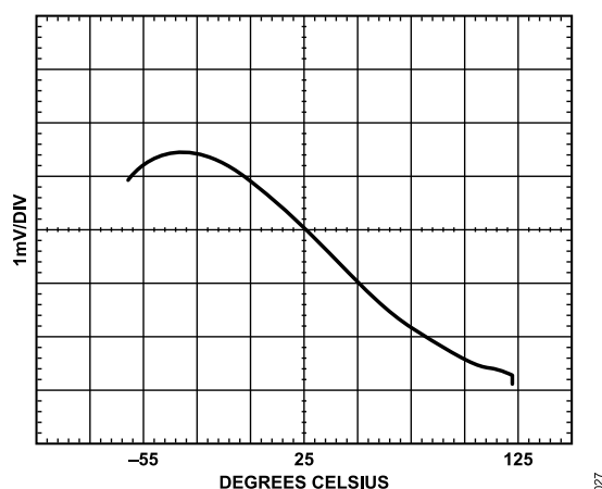
Figure 17. Reference Drift
