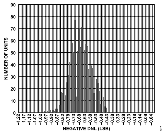
Figure 27. Typical Negative DNL Distribution (999 Units)
