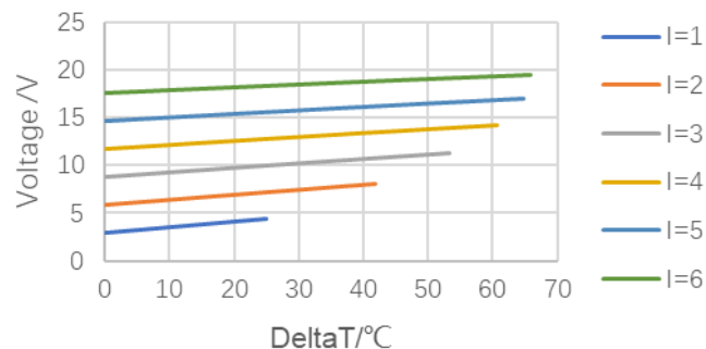
Performance Curves at T_h = 27^\circ\text{C}
