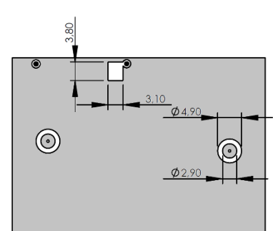
Bottom layer. Clearance through all layers. Pad 6 and 7 have identical layout as top layer and are connected by via
