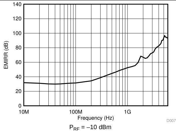
Figure 37. Electromagnetic Interference Rejection Ratio Referred to Noninverting Input (EMIRR+) vs Frequency
