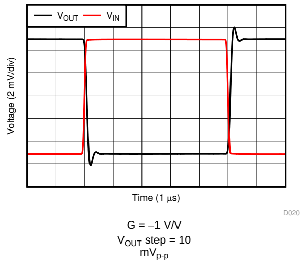
Figure 24. Small-Signal Step Response
