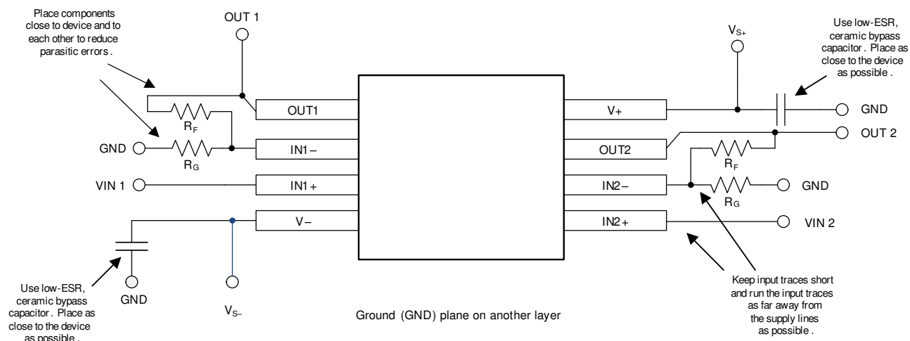
Figure 45. Layout Example
