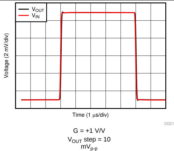
Figure 23. Small-Signal Step Response
