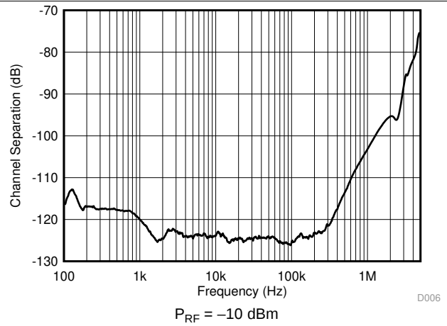
Figure 38. Channel Separation vs Frequency
