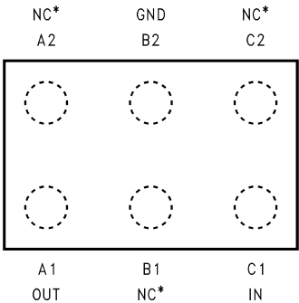
Figure 6. 6-Bump DSBGA Top View (Bump Side Down)
