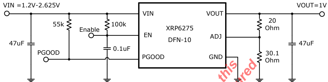
Fig. 15: XRP6274/5 Typical Application Diagram
