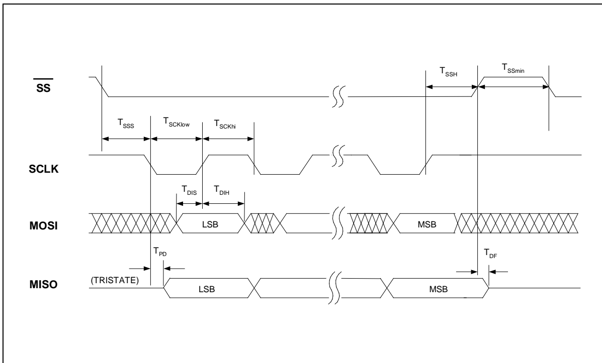
Figure 12.15: SPI Operation
