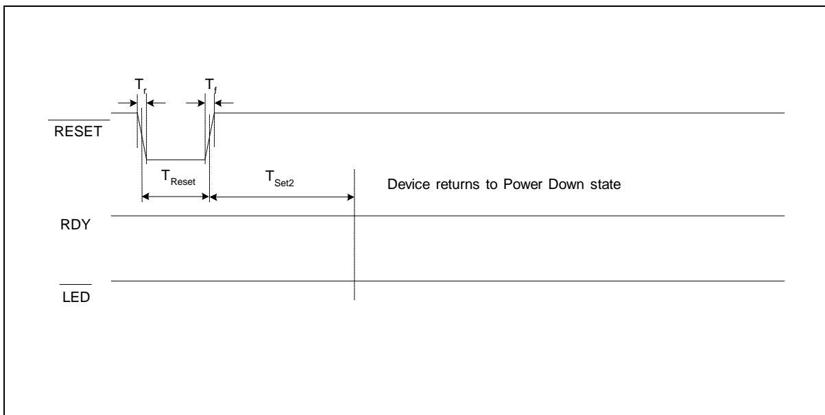
Figure 12.10: Reset Operation
