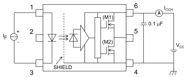
Fig. 13.1.5 I CCH Test Circuit
