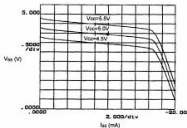
Figure 9. Band Switch Driver Output Voltage (BS1-BS4)
