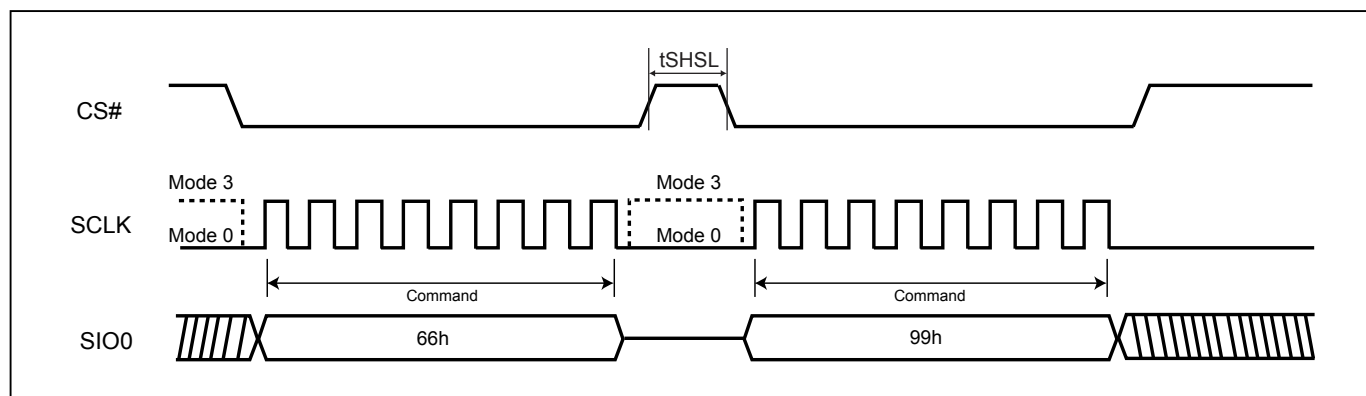
Figure 36. Reset Sequence
