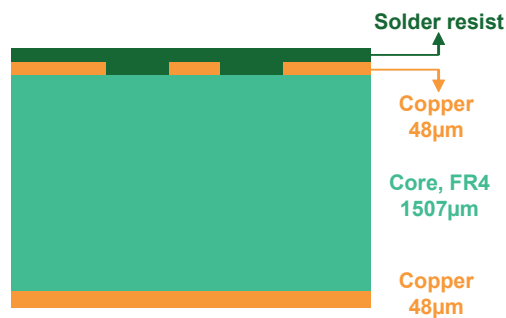
Figure 10. PCB stack-up recommendations
