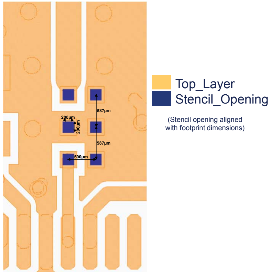
Figure 11. Stencil opening recommendations
