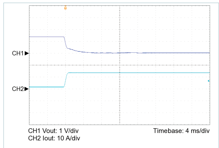
Figure 8 — 10% to 100% load transient response, V_{IN} = 275\text{ V} , nominal trim, C_{OUT\_EXT} = 200\text{ }\mu\text{F}
