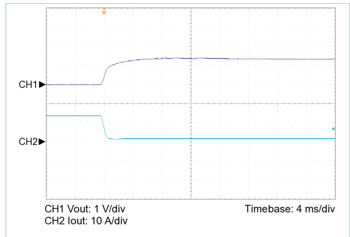
Figure 7 — 100% to 10% load transient response, V_{IN} = 275\text{ V} , nominal trim, C_{OUT\_EXT} = 200\text{ }\mu\text{F}
