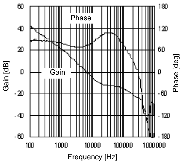
Figure 38. Gain vs Frequency 3 ( V_{CC}=5.0V, I_o=900mA )
