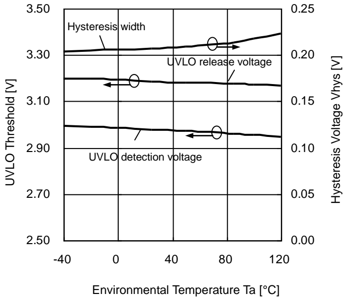
Figure 10. UVLO Threshold vs Environmental Temperature (UVLO Threshold)
