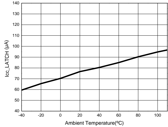
Latch Off Current vs Ambient Temperature
