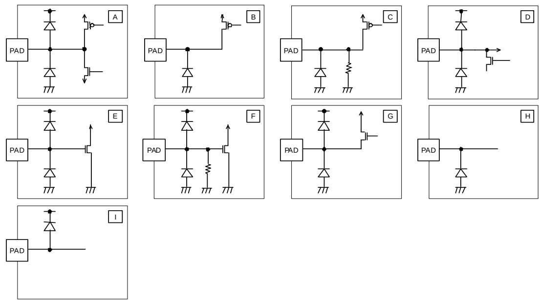
Fig.14 Pin Diagram
