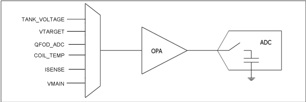
Figure 17. ADC equivalent input circuit
