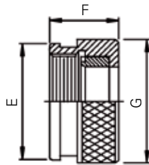
Shrink boot adapter (non removable) Type 60-2G
