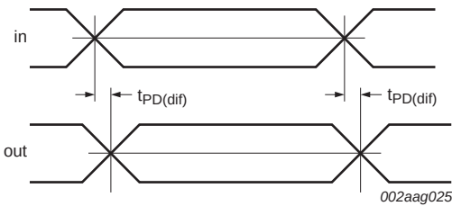
Fig 3. Propagation delay
