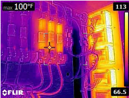
Check newly-installed electrical wiring
