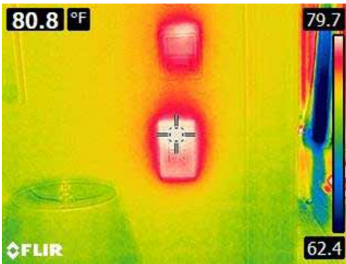
Thermostat reads a higher room temperature because of heat from the light switch below
