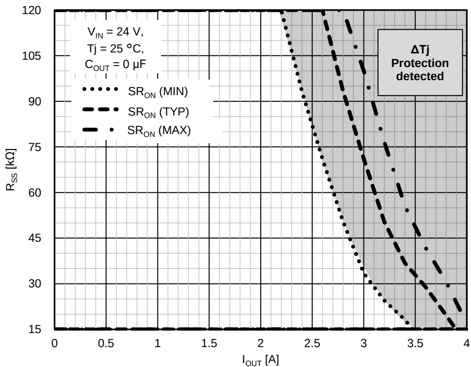
Figure 51. \Delta T_j protection function detection region at startup ( V_{IN} = 24 V, C_{OUT} = 0 \mu F)
