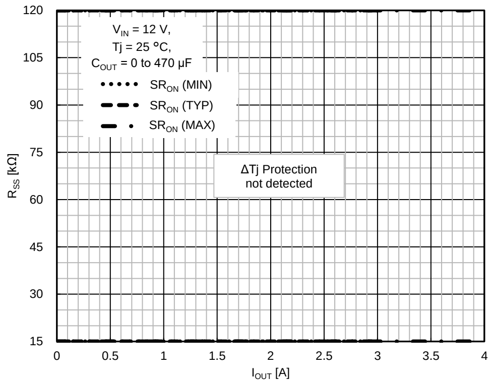
Figure 50. \Delta T_j protection function detection region at startup ( V_{IN} = 12 V, C_{OUT} = 0 to 470 \mu F)
