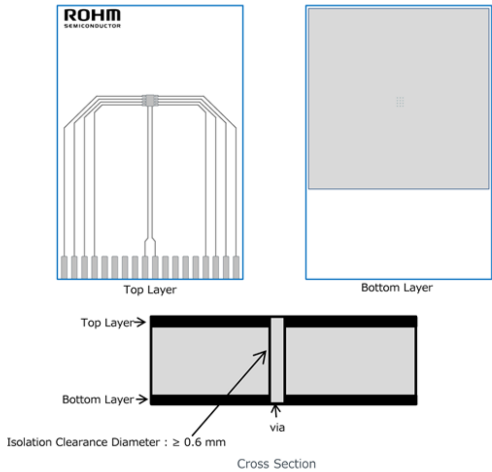
Figure 3. PCB Layout 2 Layers (2s)
