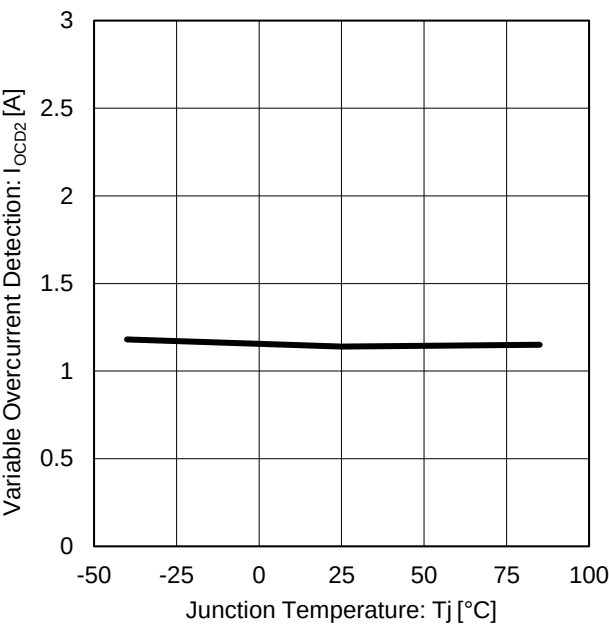
Figure 27. Variable Overcurrent Detection vs Junction Temperature
