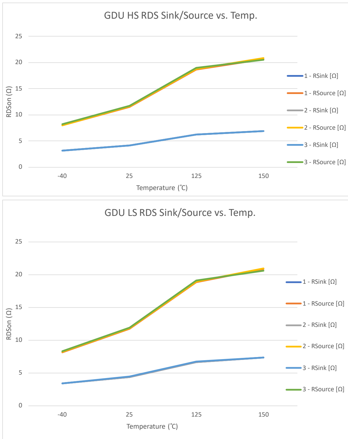
Figure 7-5. Gate Driver Unit Sink/Source ON Resistance vs Temperature
