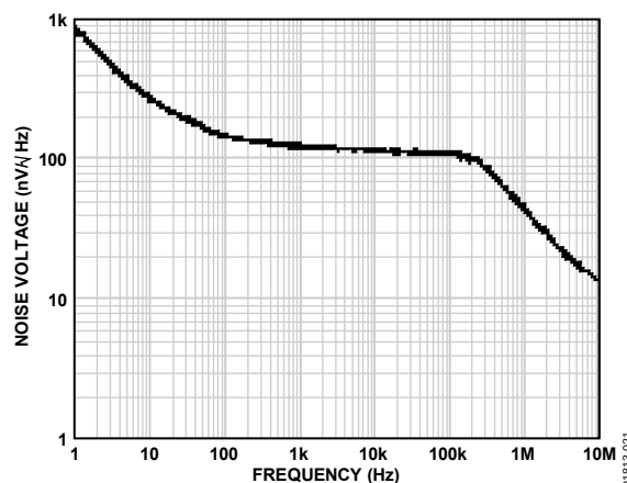
Figure 21. DAC Output Noise Voltage Spectral Density
