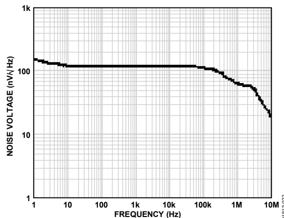
Figure 22. Reference Noise Voltage Spectral Density
