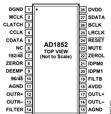
Figure 2. Pin Configuration
