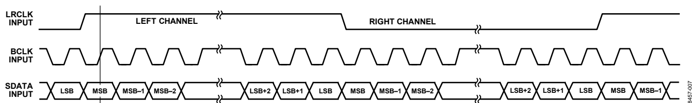
Figure 7. 32 x f s Packed Mode
