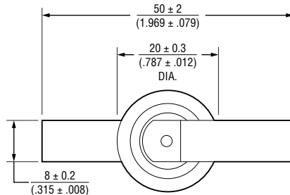
GDT220E-xx-T1
