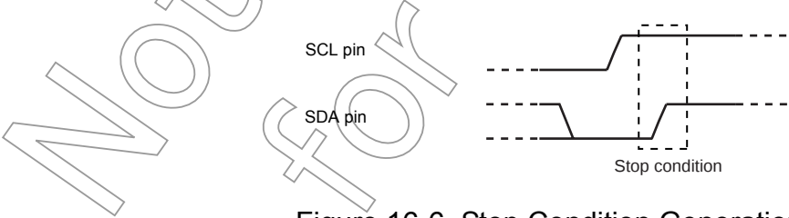
Figure 16-6 Stop Condition Generation
