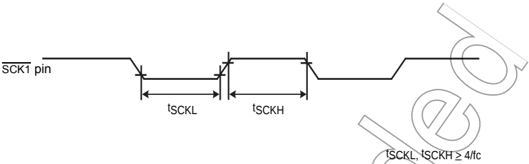
Figure 14-3 External Clock
