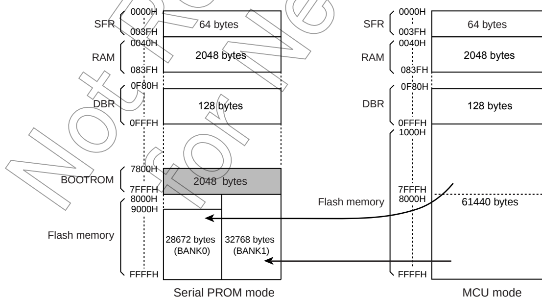
Figure 20-1 Memory Address Maps
