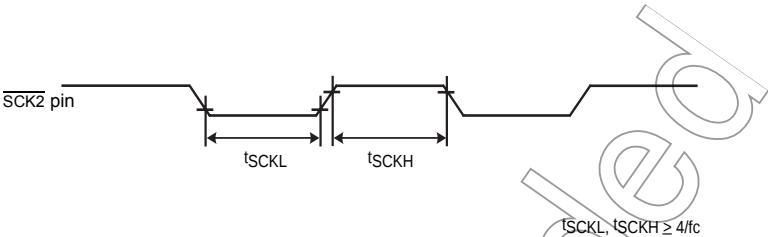
Figure 15-3 External Clock
