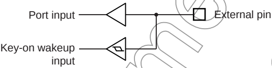
Figure 18-2 Key-on Wakeup Input and Port Input
