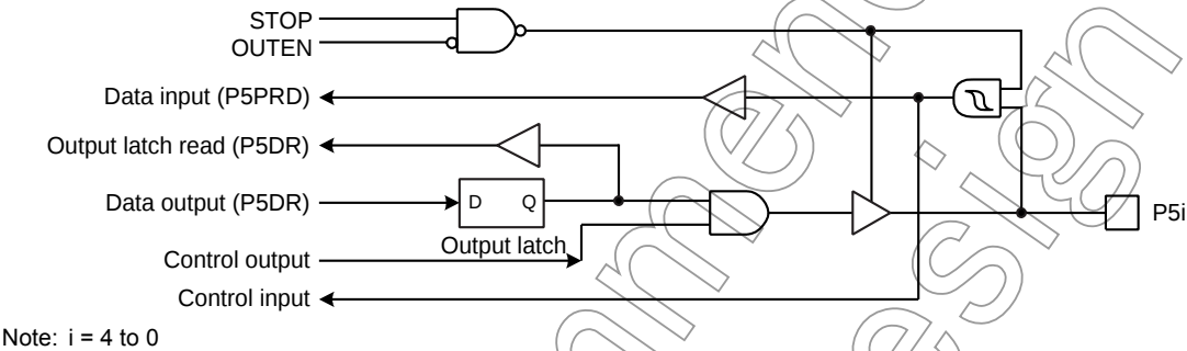
Figure 5-7 Port 5
