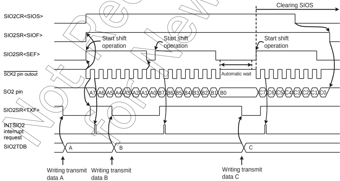
Figure 15-6 Example of Internal Clock and MSB Transmit Mode
