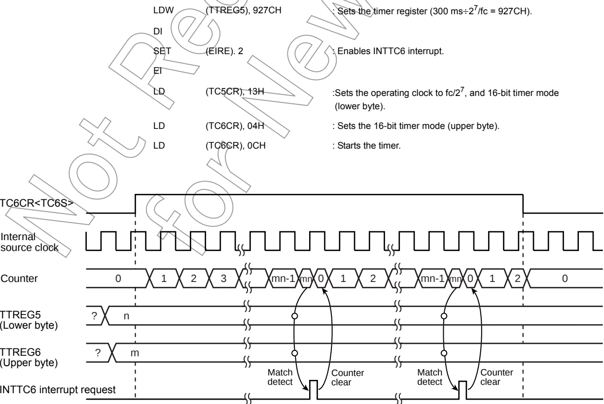
Figure 11-6 16-Bit Timer Mode Timing Chart (TC5 and TC6)
