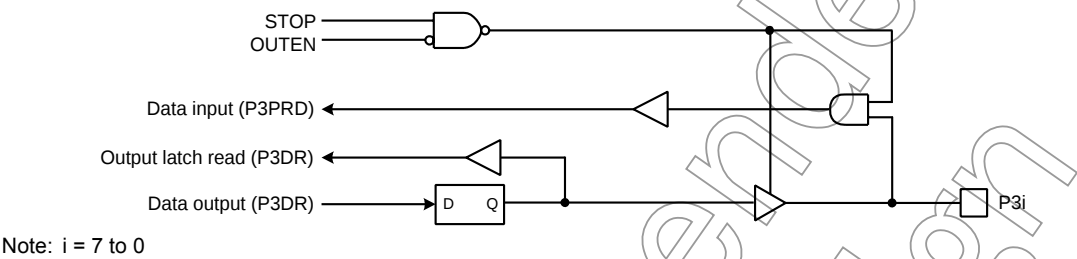
Figure 5-5 Port 3
