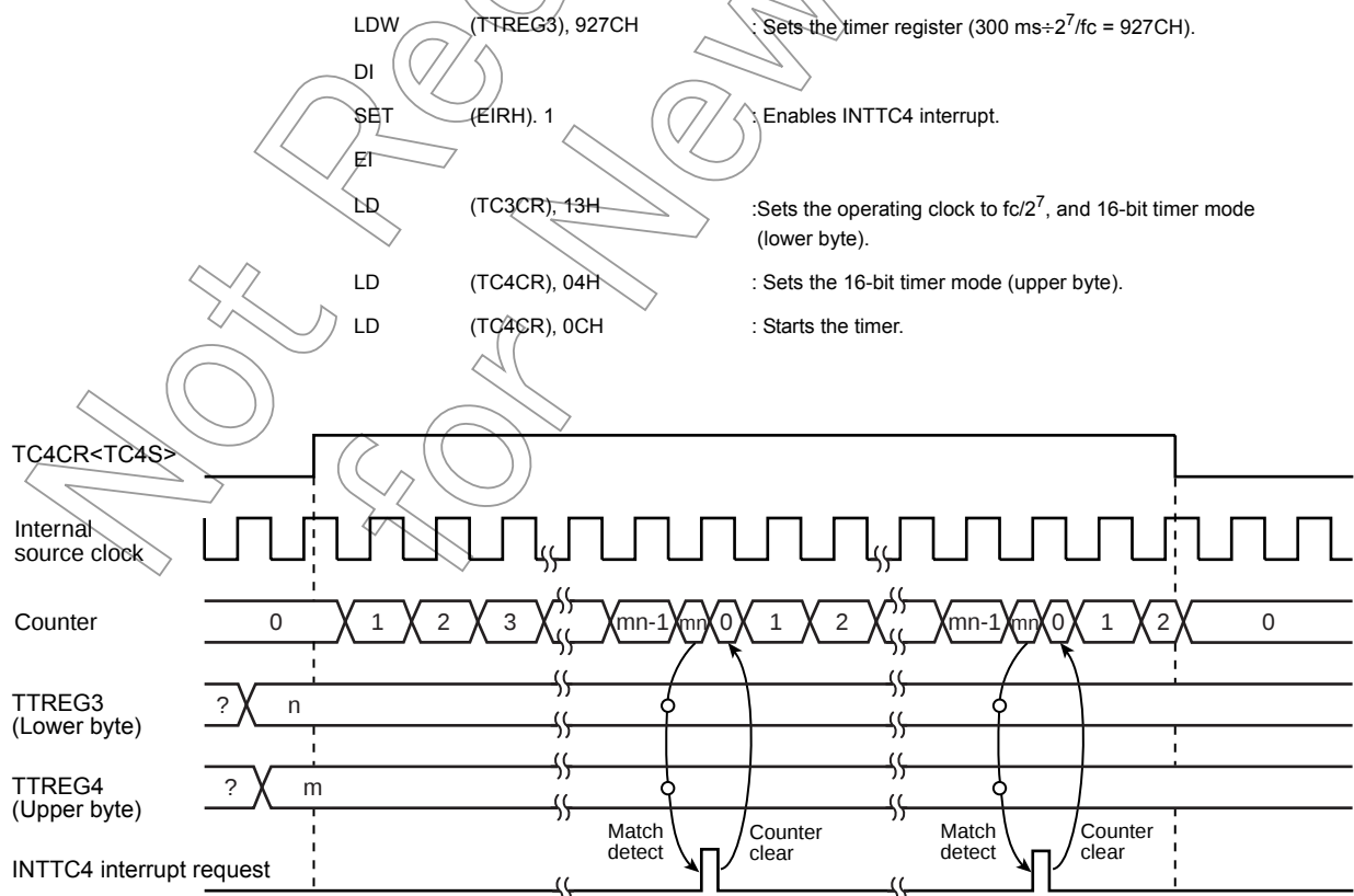
Figure 10-6 16-Bit Timer Mode Timing Chart (TC3 and TC4)
