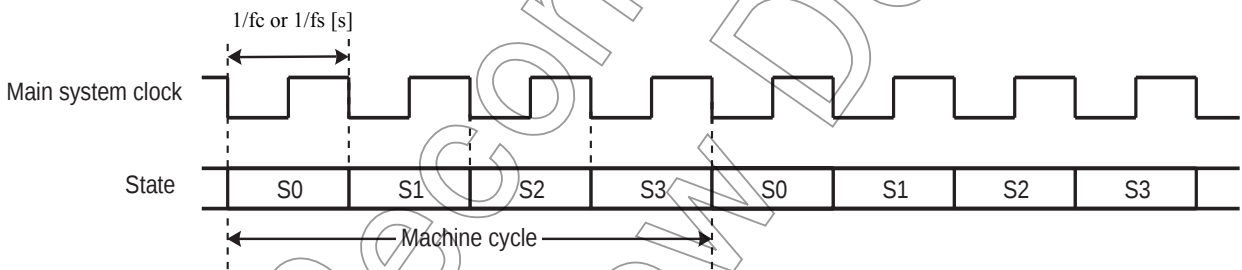
Figure 2-5 Machine Cycle
