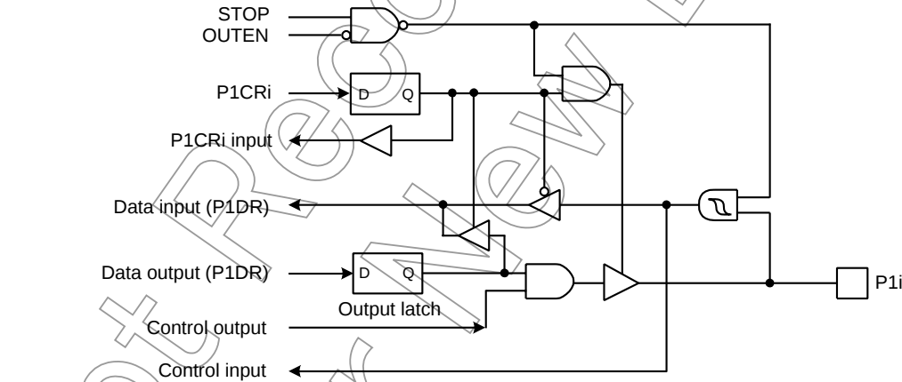
Figure 5-3 Port 1 and P1CR
