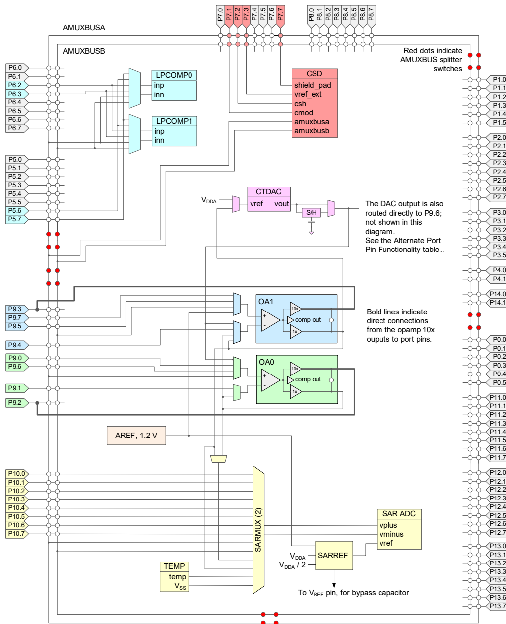
Figure 7. Analog Subsystem
