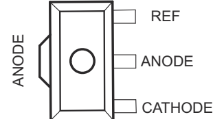
TL432, TL432A, TL432B ... PK (SOT-89) PACKAGE (TOP VIEW)
