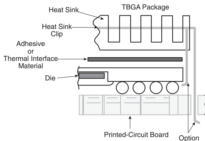
Figure 1-6. Package-Exploded Cross-Sectional View with Several Heat Sink Options
