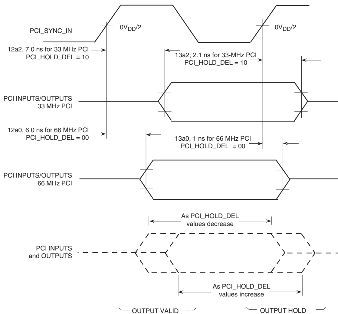
Figure 2-10. PCI_HOLD_DEL Effect on Output Valid and Hold Time
