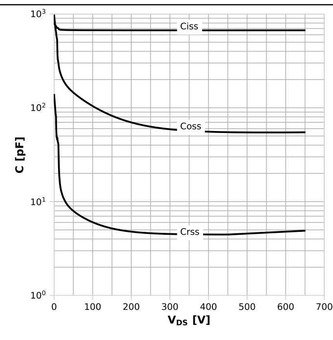
Diagram 15: Typ. capacitances
