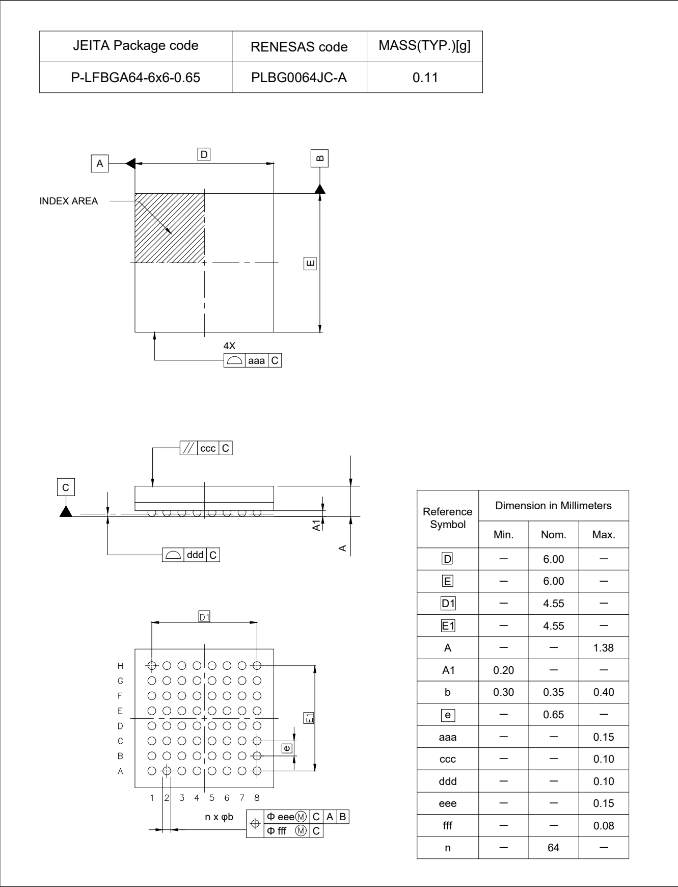
Figure A2.4 BGA 64-pin
