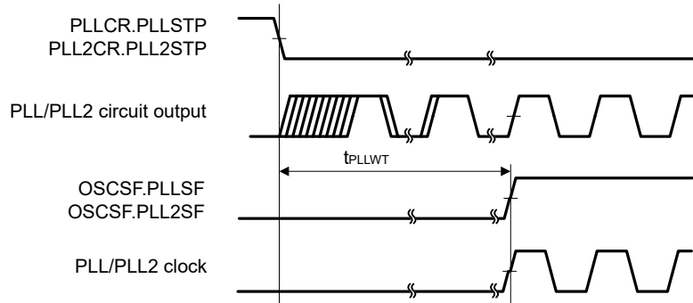
Figure 2.11 PLL/PLL2 clock oscillation start timing
