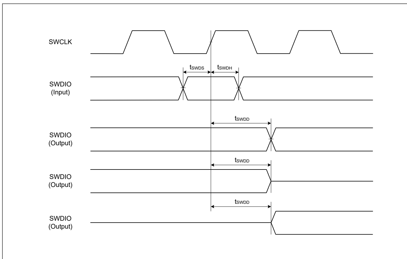
Figure 2.94 SWD input/output timing
