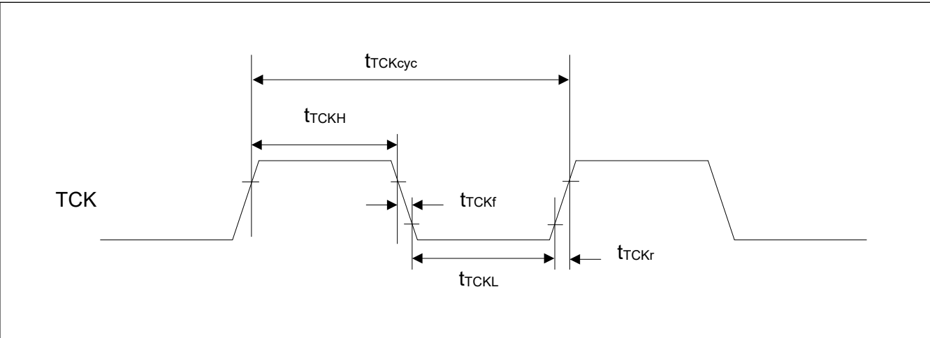
Figure 2.91 JTAG TCK timing
