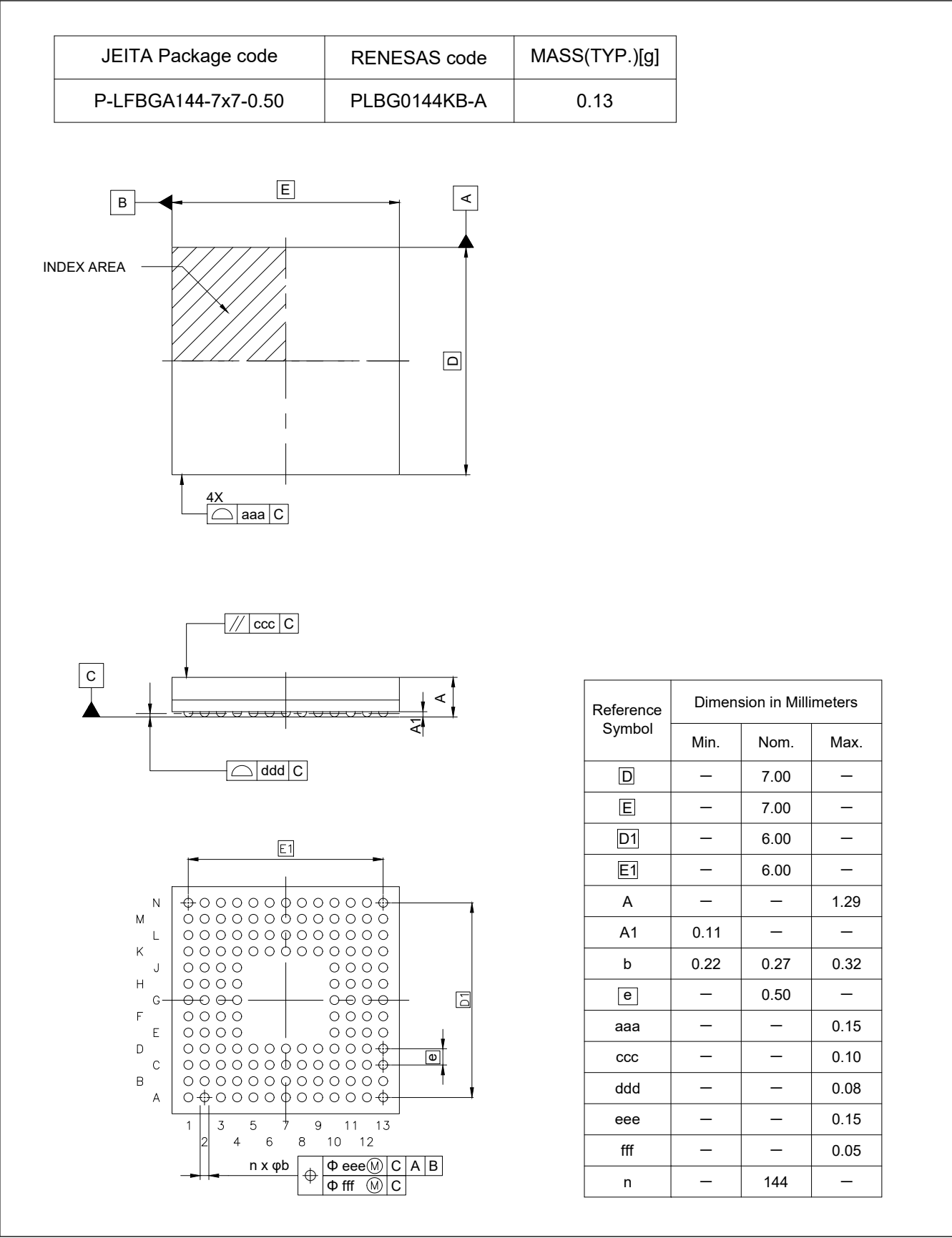
Figure A2.5 BGA 144-pin
