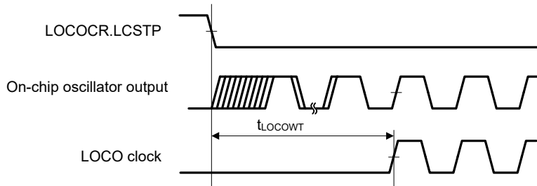
Figure 2.10 LOCO clock oscillation start timing
