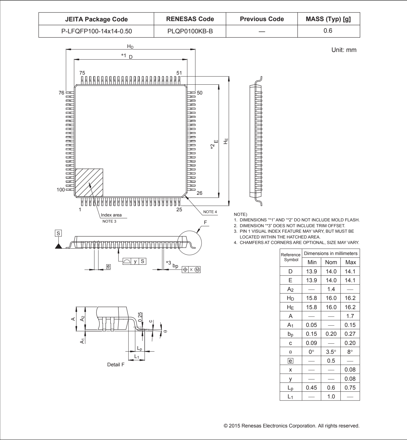
Figure A2.2 LQFP 100-pin
