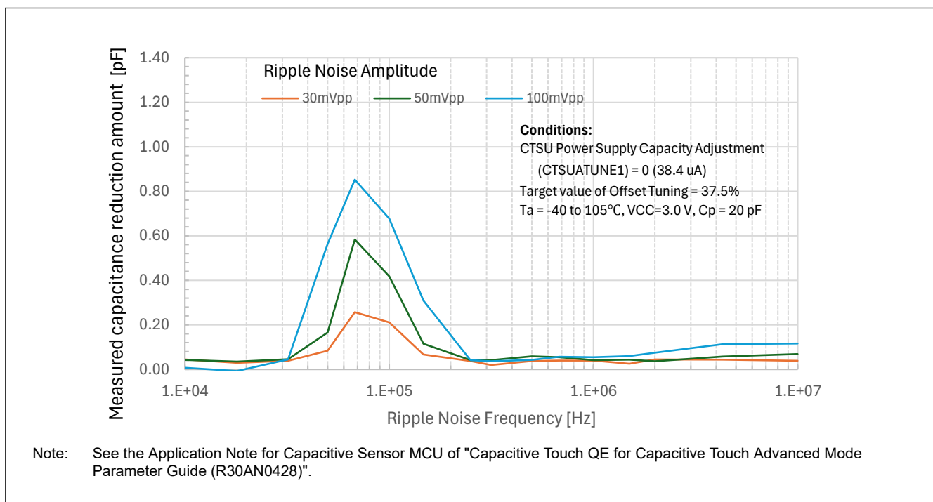
Figure 2.86 Measured capacitance reduction amount
