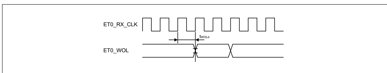
Figure 2.73 WOL output timing for MII
