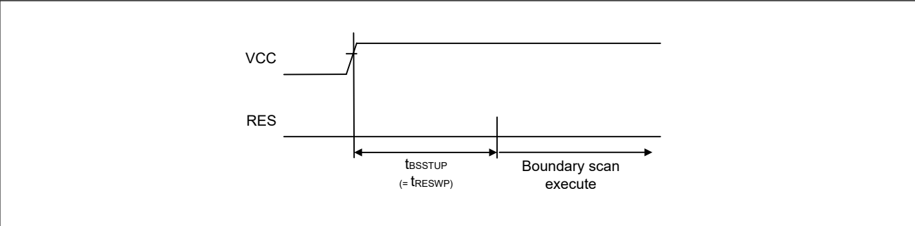
Figure 2.90 Boundary scan circuit startup timing
