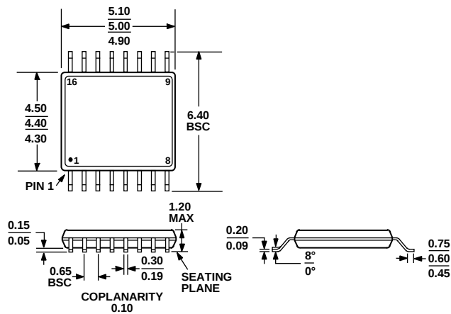
Figure 10. 16-Lead Thin Shrink Small Outline Package [TSSOP] (RU-16) Dimensions shown in millimeters
