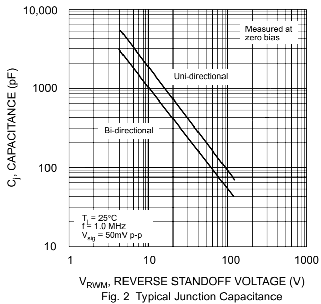
Fig. 2 Typical Junction Capacitance
